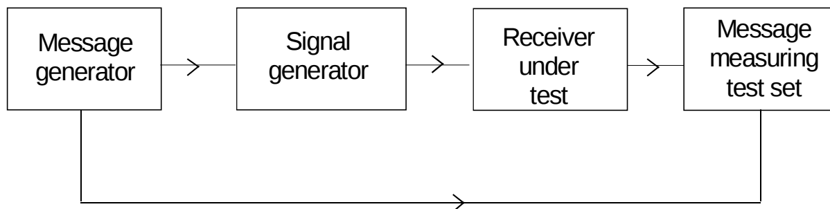
Figure 9: Measurement arrangement
